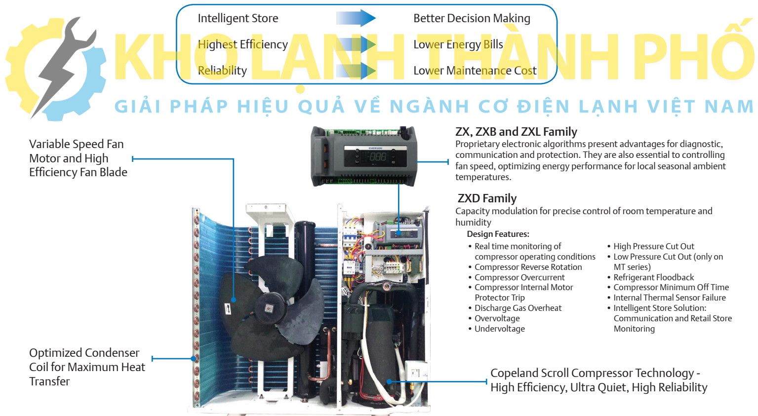
Figure 1. ZX Platform CDU Features
